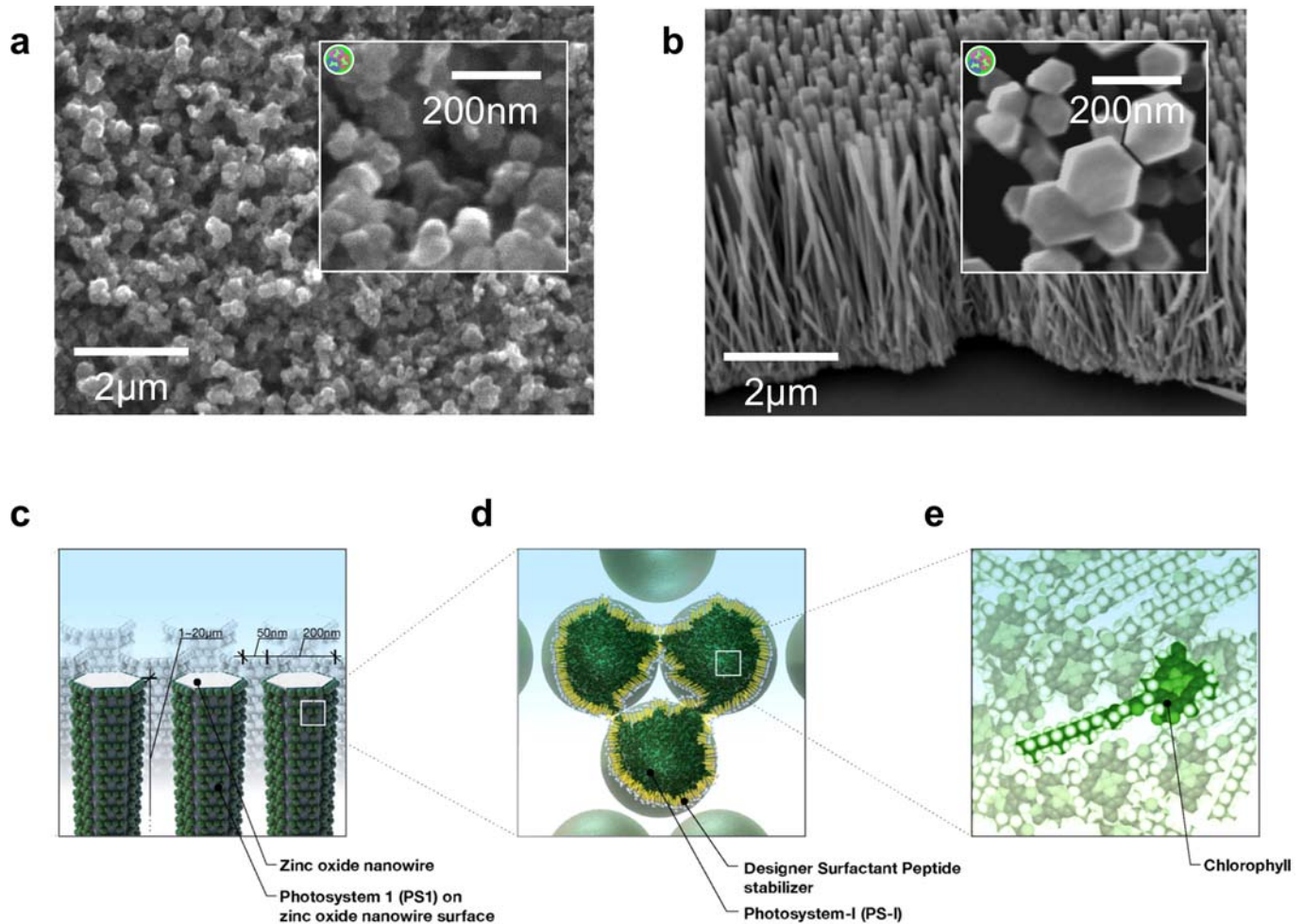
Figure 3 | SEM of nanostructured TiO 2 and ZnO photoanodes and schematic of an ideal ultra-low cost biophotovoltaic arrangement. (a) 3.8 μm-thick, 60 nm-pore TiO 2 nanocrystalline photoanode of roughness factor \rho_{\text{TiO}_2} \sim 200 (i.e. surface area increases by roughly fifty times per μm of film thickness) fabricated as described previously 13 . (b) 3 μm tall, ZnO nanowires grown on Zn-nanoparticle-seeded ITO-glass as described elsewhere 15 , \rho_{\text{ZnO}} \sim 30 . Round graphic at top left of inserts represents a PS-I trimer drawn to scale. (c), (d), (e) ideal arrangement of PS-I and designer surfactant peptide stabilizers on ZnO nanowires that could be grown at room temperature on a variety of flexible and inexpensive substrates 16 .
